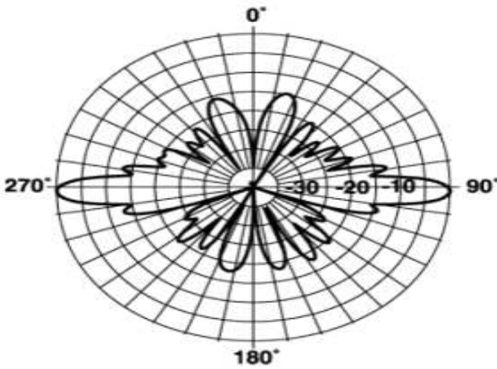
Vertical Pattern
